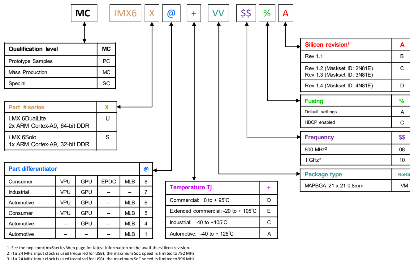
Figure 1. Part Number Nomenclature—i.MX 6Solo and 6DualLite
