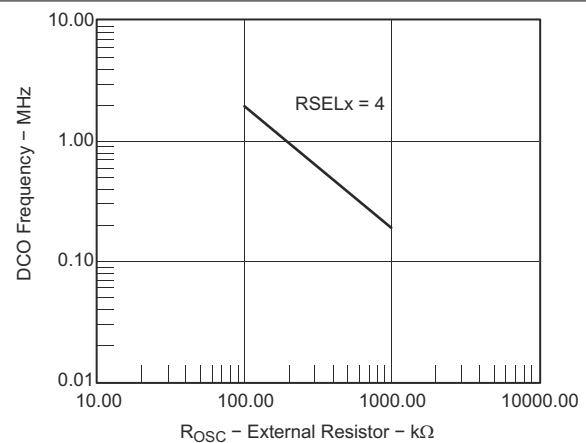
Figure 8-20. DCO Frequency vs R_{OSC} (V CC = 3 V, T A = 25°C)
