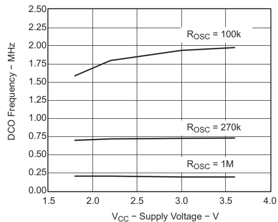
Figure 8-22. DCO Frequency vs Supply Voltage (T A = 25°C)
