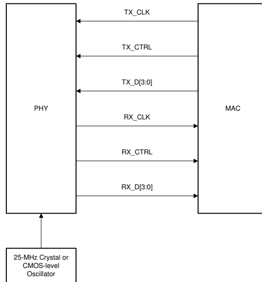
Figure 8-13. RGMII Connections
