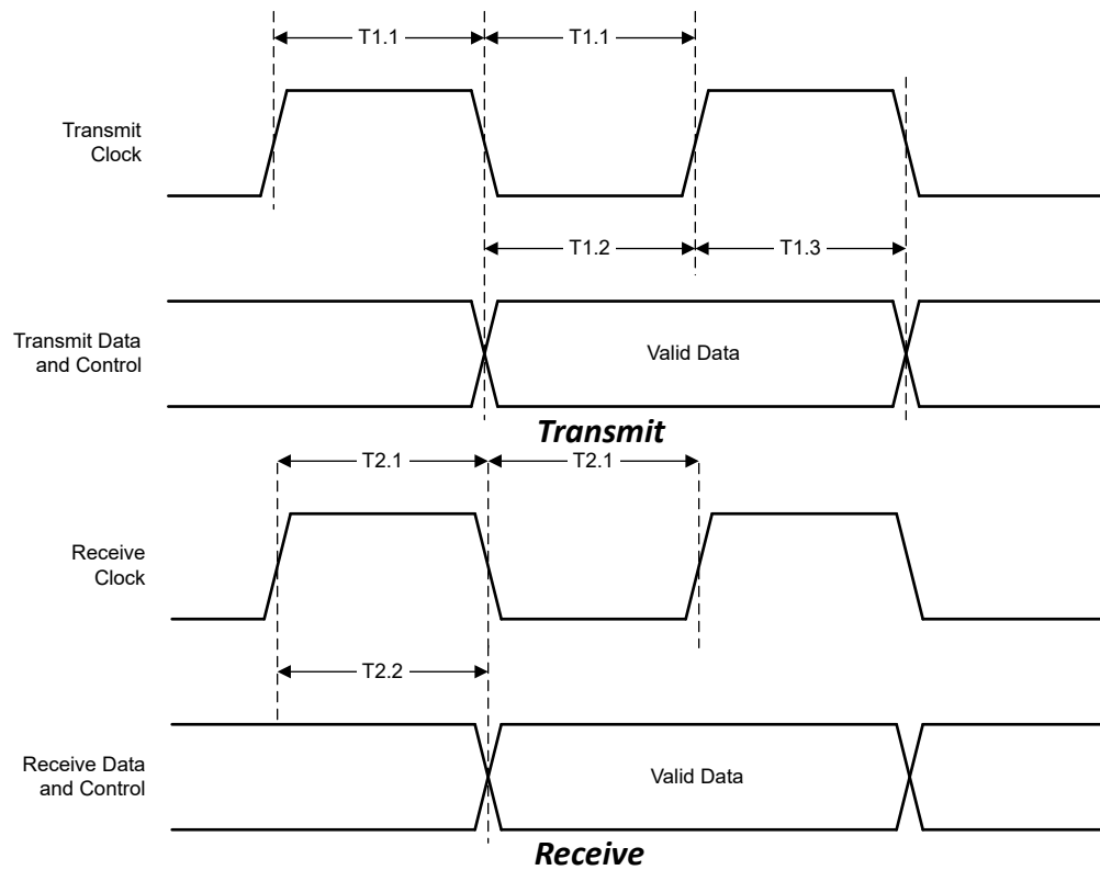
Figure 7-1. MII Timing
