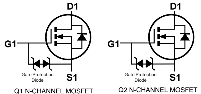
Internal Schematic
