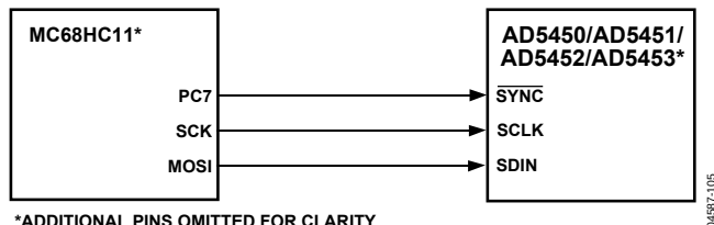
Figure 58. MC68HC11-to-AD5450/AD5451/AD5452/AD5453 Interface
