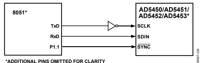
Figure 57. 80C51/80L51-to-AD5450/AD5451/AD5452/AD5453 Interface
