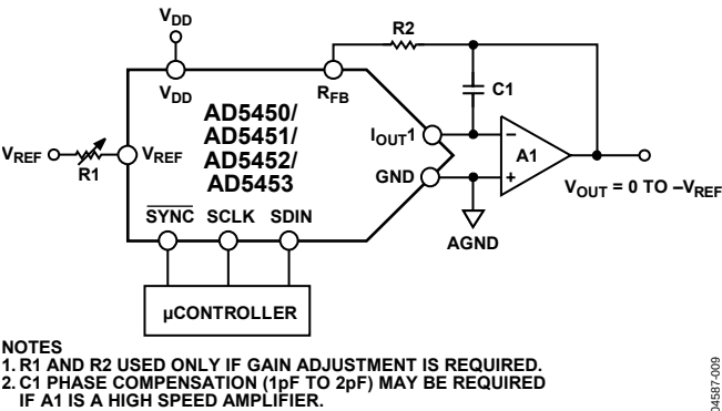
Figure 43. Unipolar Mode Operation
