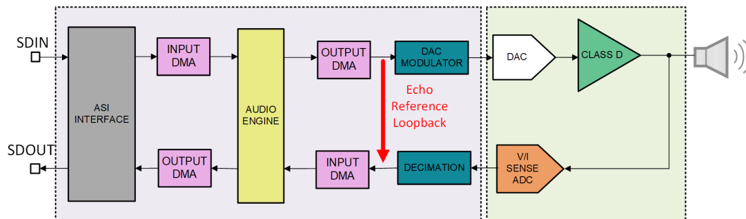
Figure 8-10. Echo Reference Loopback
