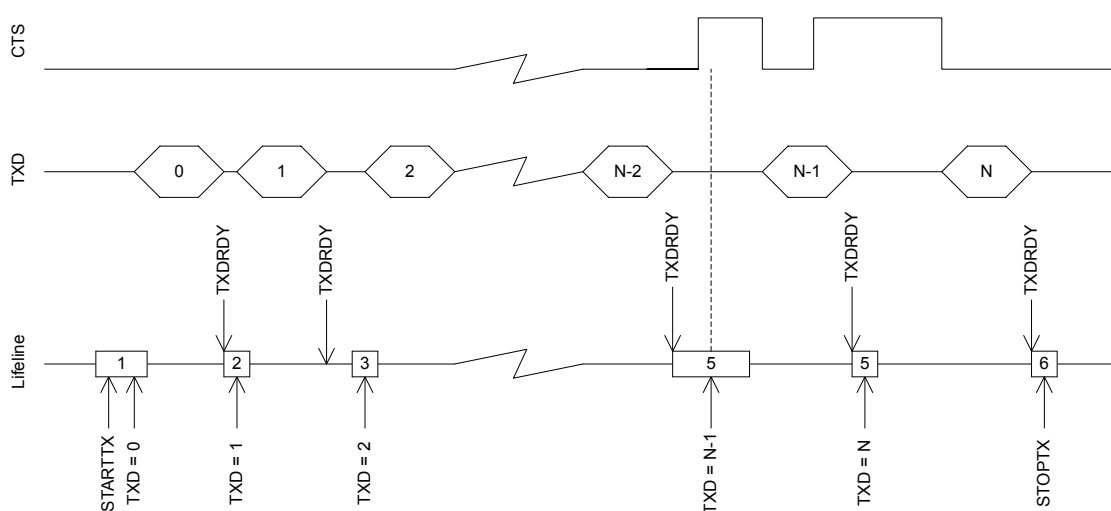
Figure 131: UART transmission
