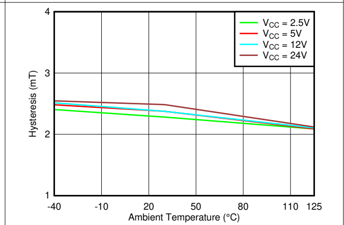
Figure 7-6. Hysteresis Z vs. Temperature
