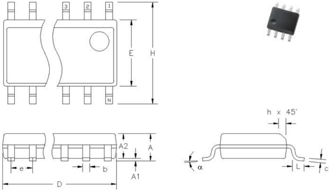
Figure 6: Package drawing
