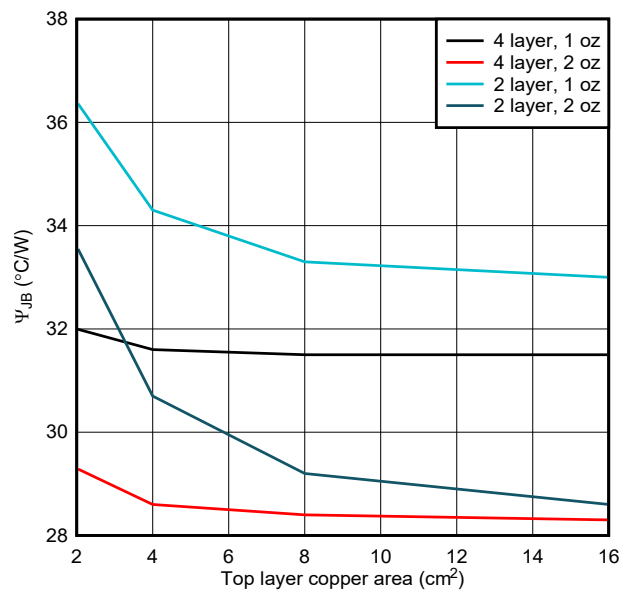
Figure 9-15. WSON, junction-to-board characterization parameter vs copper area
