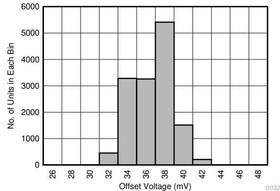
14000 devices, \mu = 35.7\text{ mV} , \sigma = 2.15\text{ mV} Figure 7-24. Offset Voltage Distribution Histogram
