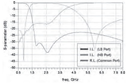
RFDIP2520100G2T
