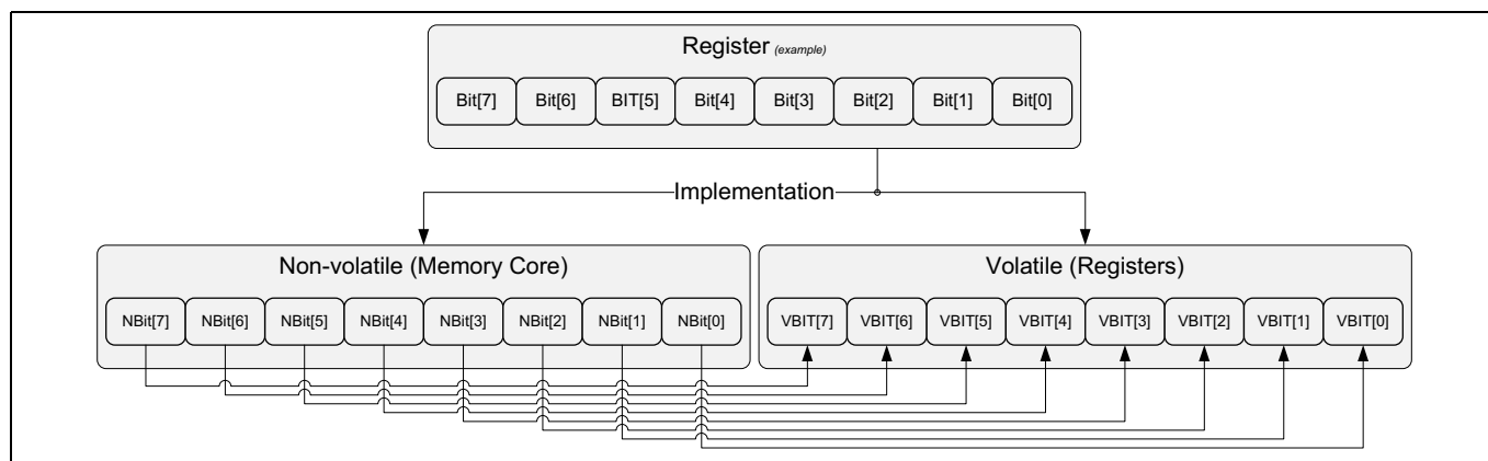
Figure 50 Register structure
