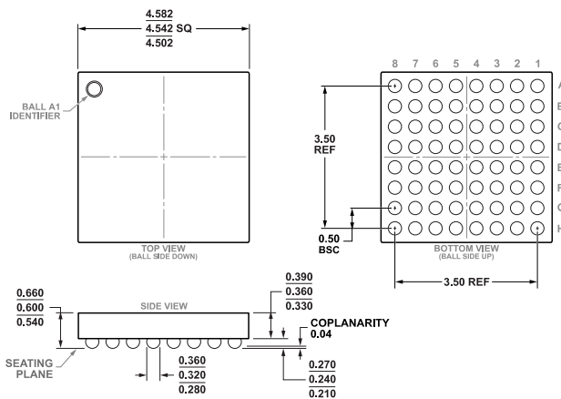
Figure 62. 64-Ball Wafer Level Chip Scale Package [WLCSF] (CB-64-5)
