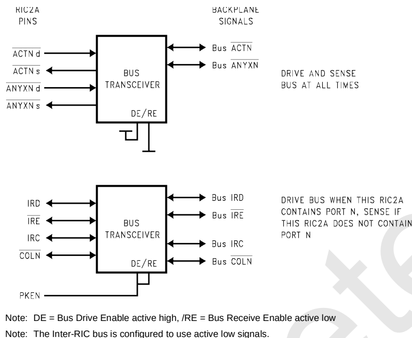
Figure 10. External Bus Transceiver Connection Diagram
