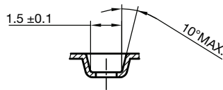
B-B Section
