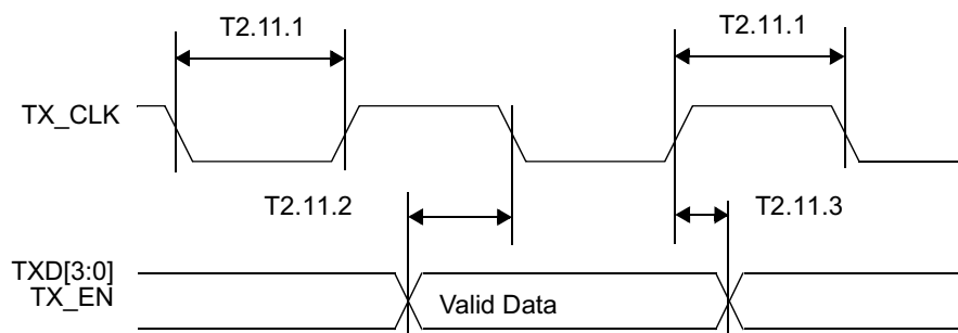
Figure 4-11. 10 Mb/s MII Transmit Timing
