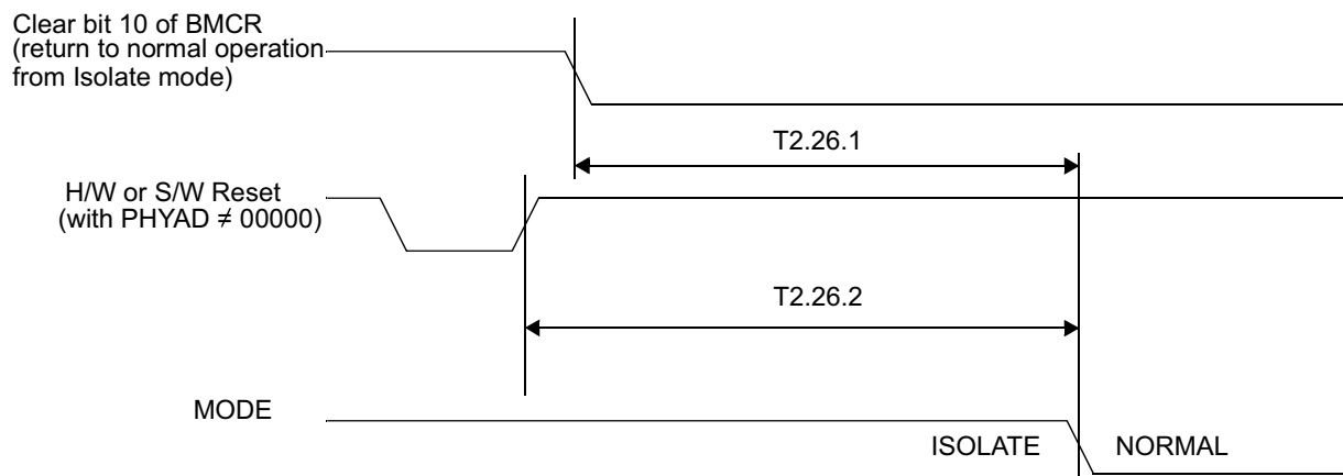
Figure 4-31. Isolation Timing
