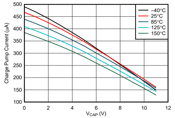
Figure 6-4. Charge Pump V-I Characteristics at V SOURCE >= 12 V
