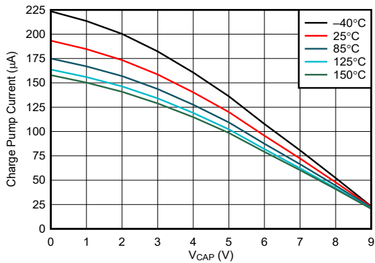
Figure 6-5. Charge Pump V-I Characteristics at V SOURCE = 3.2 V
