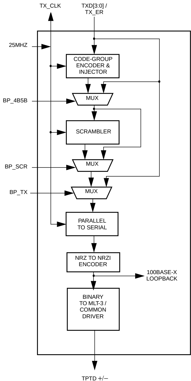
Figure 1. 100BASE-TX Transmit Block Diagram
