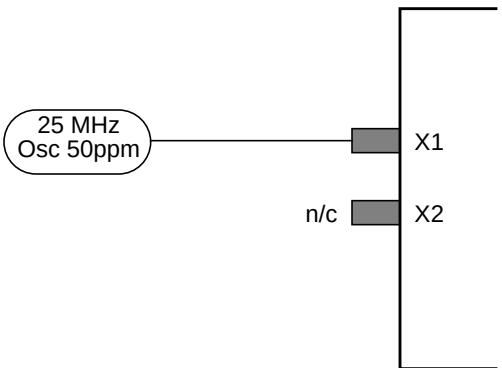
Figure 20. Oscillator Reference Clock Connection Diagram
