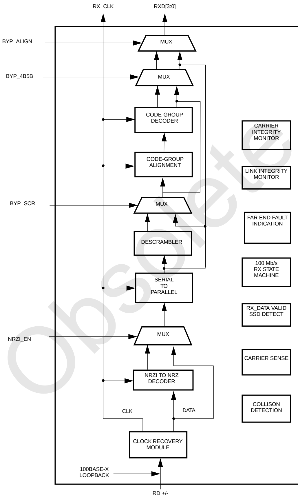
FIGURE 5. 100BASE-X Receiver
