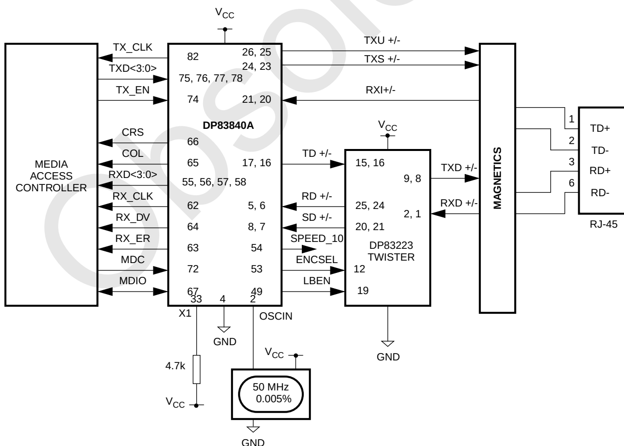
FIGURE 20. Typical 10/100 Ethernet Node Design Device Interconnection
