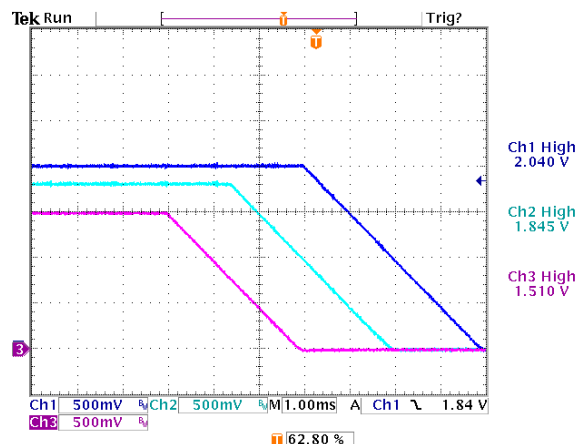
Figure 22. Turn-Off with Tracking and Sequencing. Falling Slew Rate is Programmed at 0.5V/ms. Vin=12V
