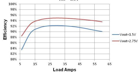
Figure 1. Efficiency at V_{in} = 8V V_{in} = 8.0V
