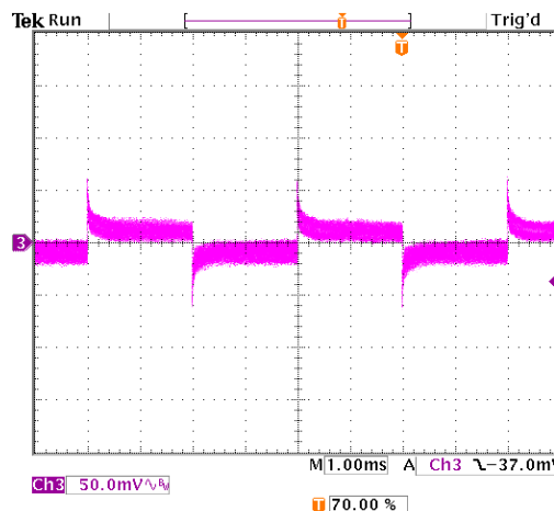
Figure 44. Transient Response with Regulation set to 3.72mV/A
