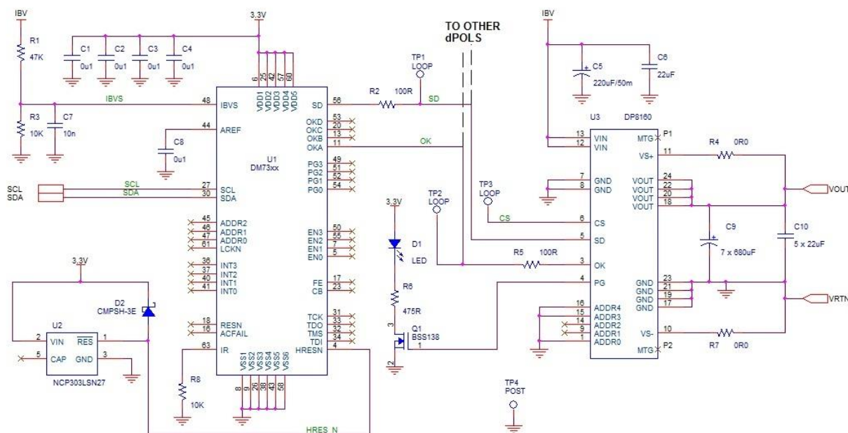
Figure 50. Block Diagram of Typical Multiple Output Application with Digital Power Manager and I 2 C Interface
