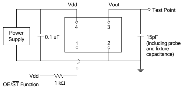
Figure 1. Test Circuit
