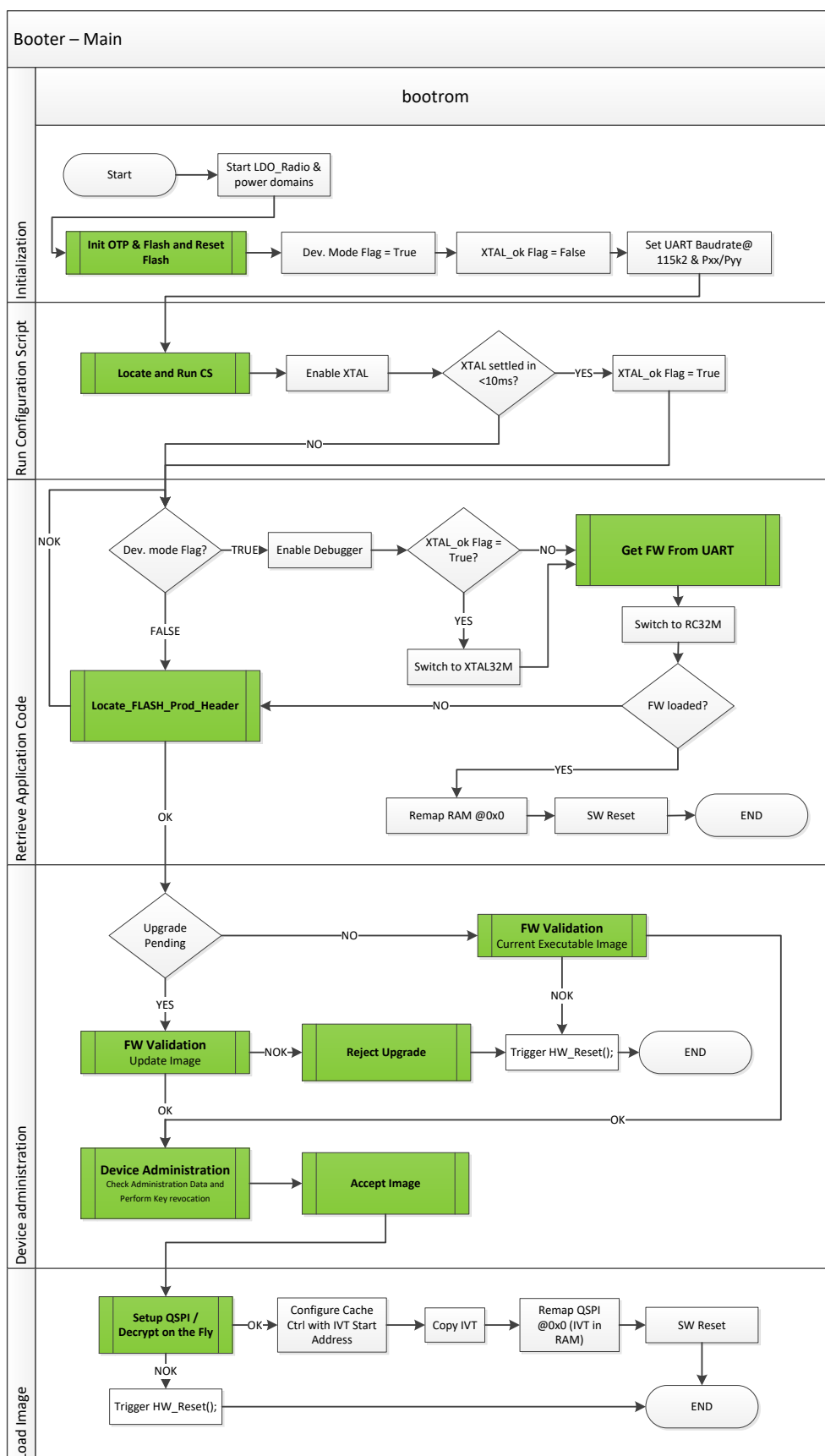
Figure 14: BootROM Flowchart
