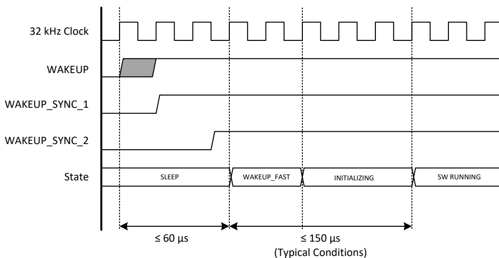
Figure 11: Fast WAKEUP Timing
