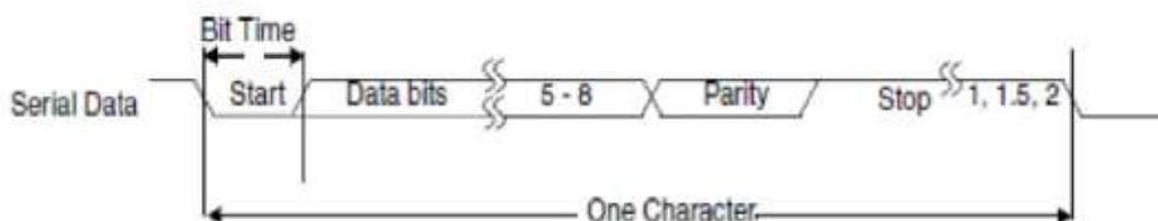
Figure 80: Serial Data Format
