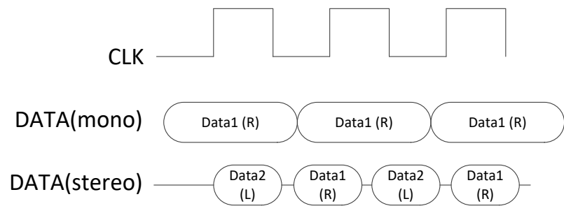
Figure 67: PDM Mono/Stereo Formats
