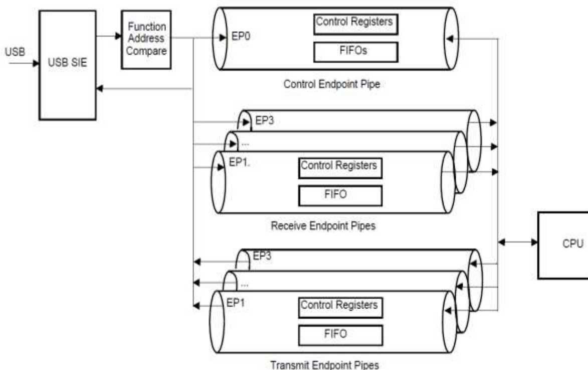
Figure 95: Endpoint Operation
