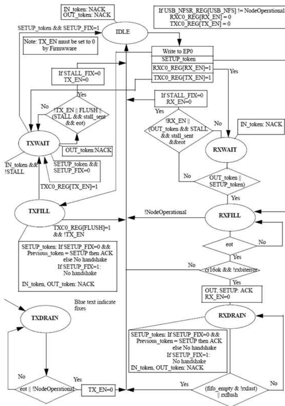
Figure 98: Endpoint 0 Operation
