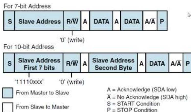
Figure 74: Master-Transmitter Protocol
