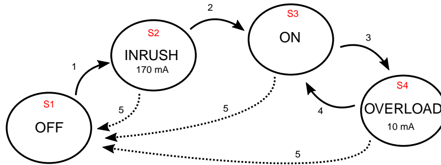
Figure 2.5. Hotswap Switch 4-State Machine
