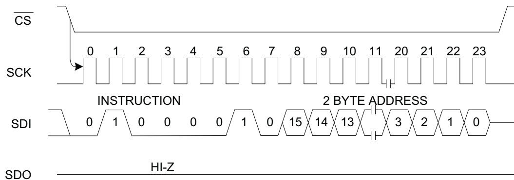
Figure 8-8. PERS Sequence
