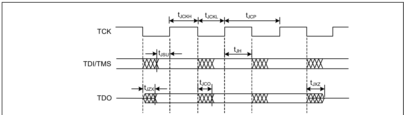
Figure 26-22 JTAG specifications
