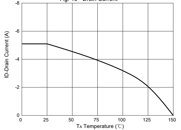
Fig. 10 - Drain Current
