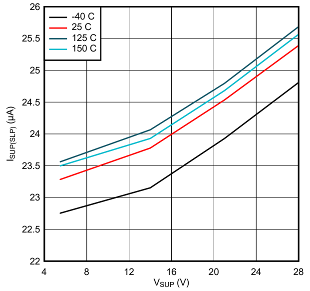
Figure 8-2. I SUP over V SUP Sleep Mode
