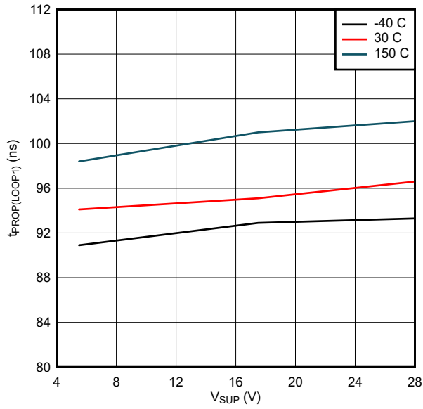
Figure 8-1. t PROP(LOOP1) over V SUP
