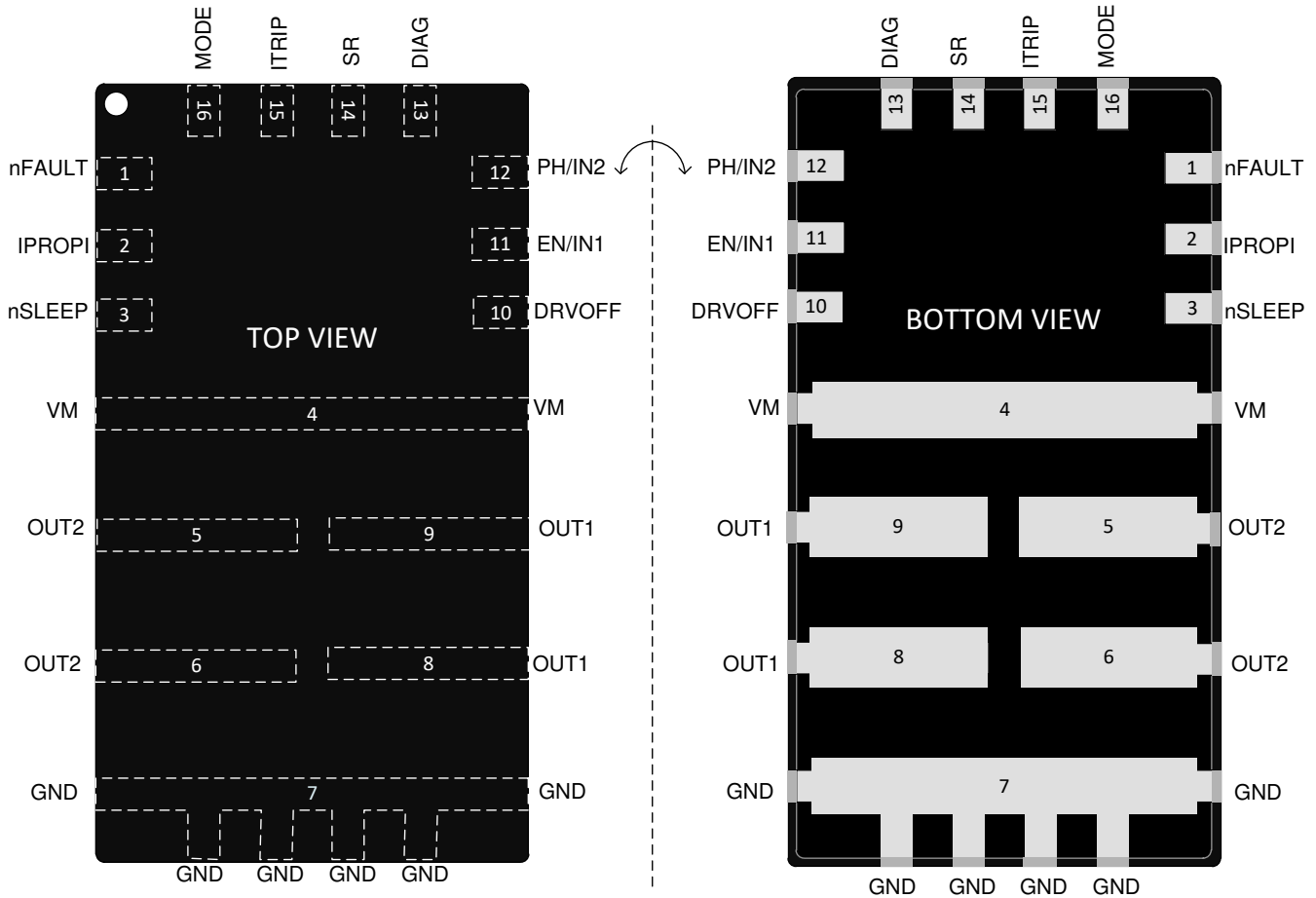
Figure 6-2. DRV8244H-Q1 HW variant in VQFN-HR(16) package
