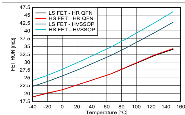
Figure 7-12. R_{HS\_ON} & R_{LS\_ON} vs Temperature at V_{VM} = 13.5 V
