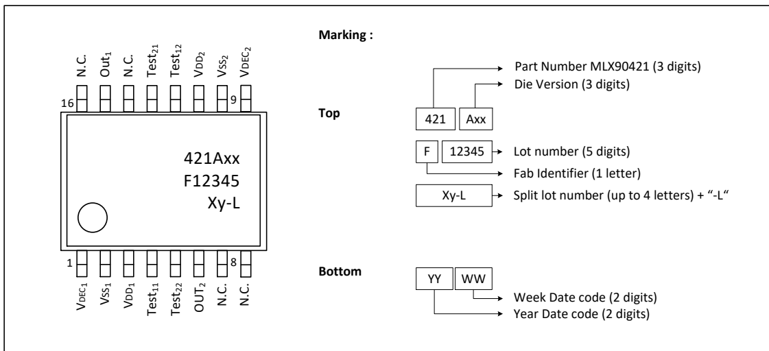
Figure 24 - TSSOP-16 pinout and marking
