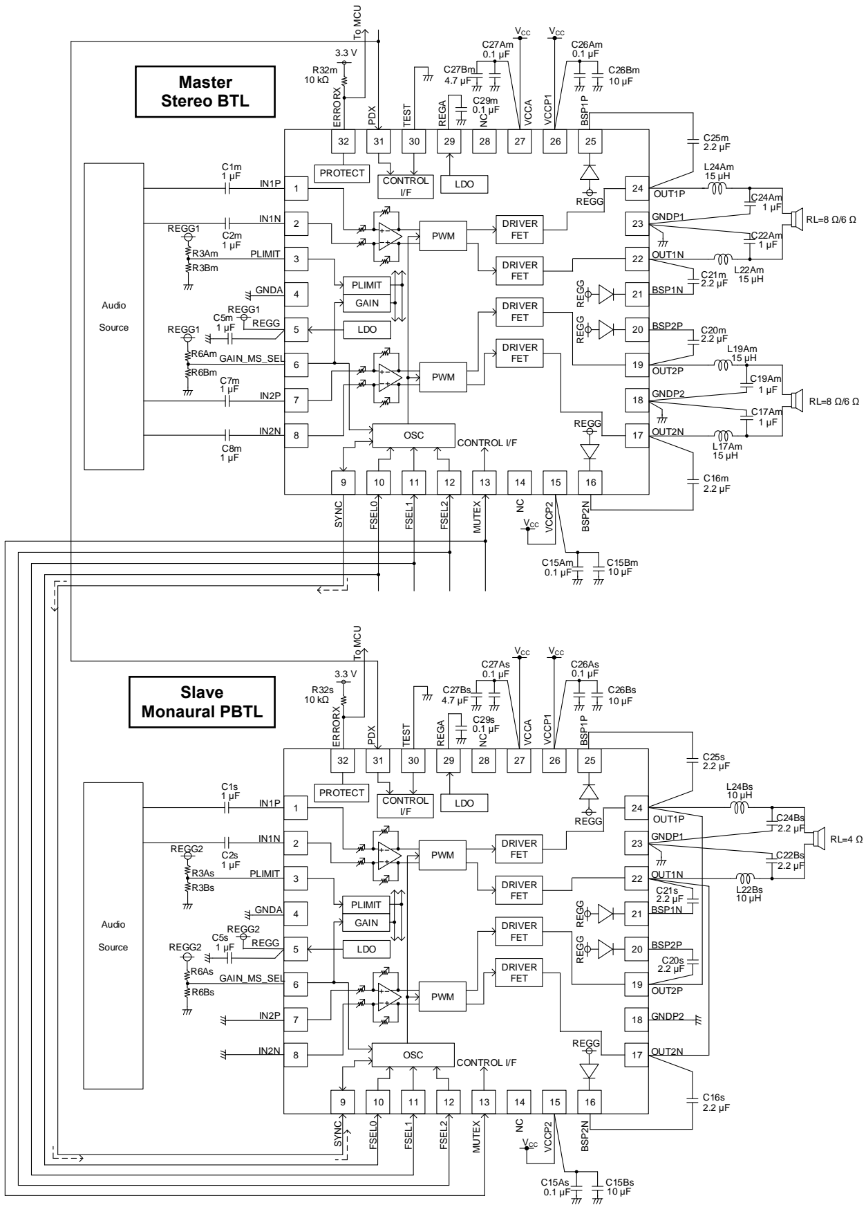
Figure 48. Application Circuit 5
