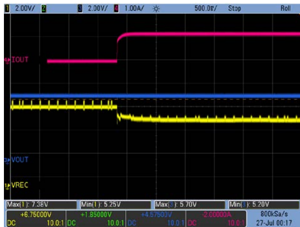
Figure 9. Load Transient: V OUT = 5.5V, 0A → 1.2A
