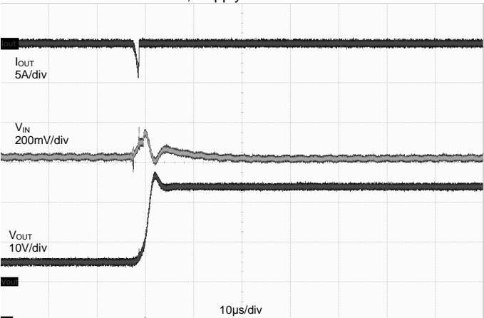
Reverse-Voltage Response V_{IN} = 5\text{V} , Supply 24V to OUT Port
