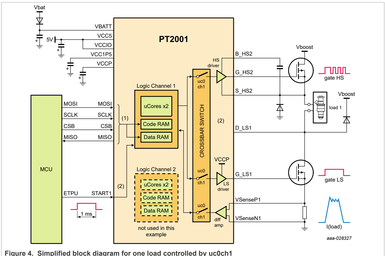
Figure 4. Simplified block diagram for one load controlled by uc0ch1
