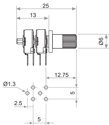
Fig. 18 - Ref: 6064 2-gang plastic knob/shaft
