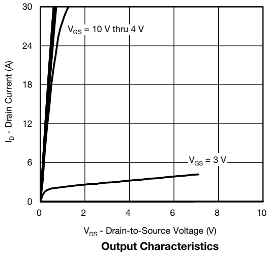
Output Characteristics
