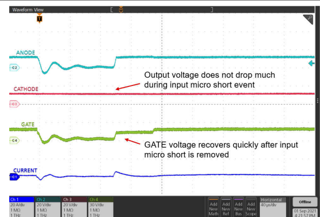
Figure 9-9. Response to LV124 E-10 (Input Micro Short, 100 µs)
