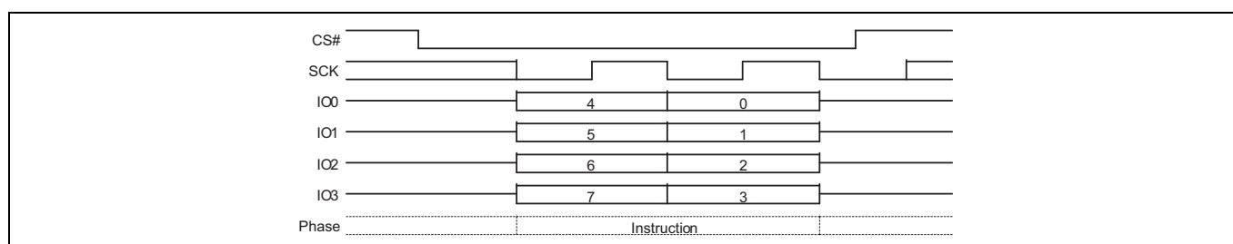
Figure 110 Mode Bit Reset command sequence QPI mode
