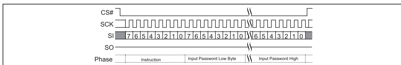
Figure 106 Password Unlock command sequence
