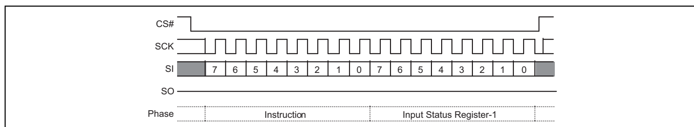
Figure 49 Write Registers (WRR) command sequence – 8 data bits
