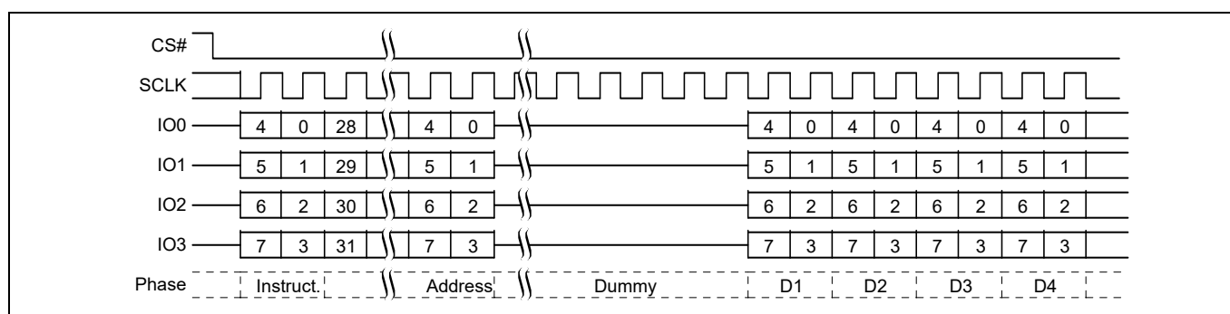
Figure 60 ECCRD (19h), QPI mode, CR2[7] = 1, or 4EECRD (18h) command sequence
