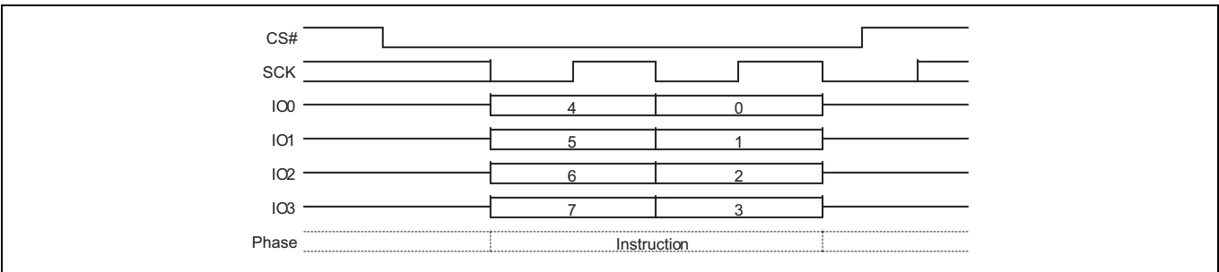
Figure 55 Write Disable (WRDI) command sequence QPI mode
