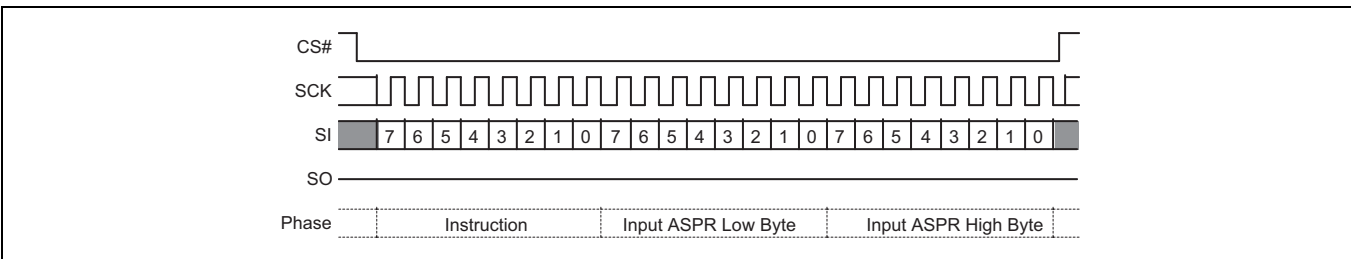
Figure 94 ASPP command
