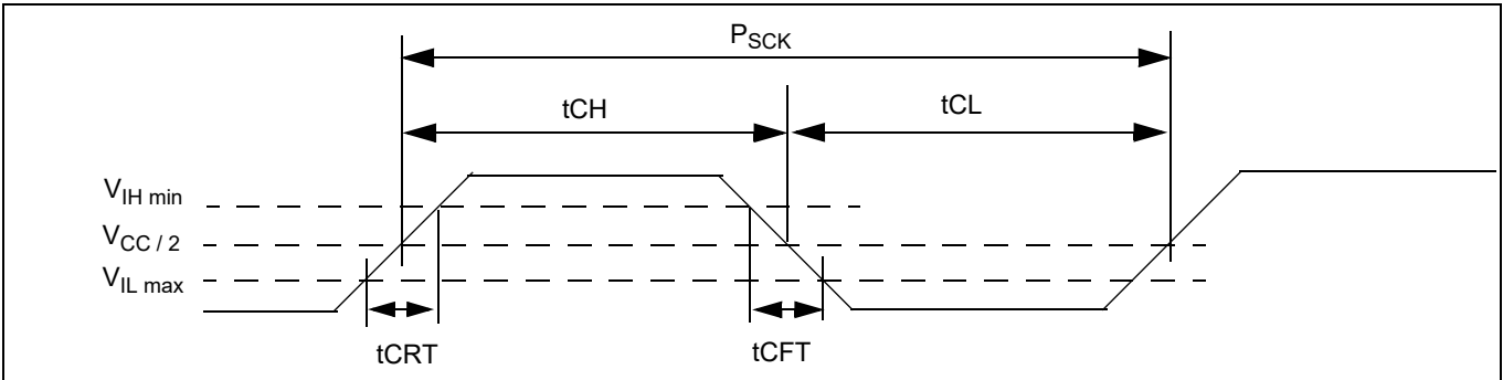
Figure 31 Clock timing
