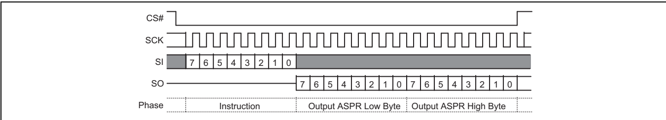
Figure 93 ASPRD command
