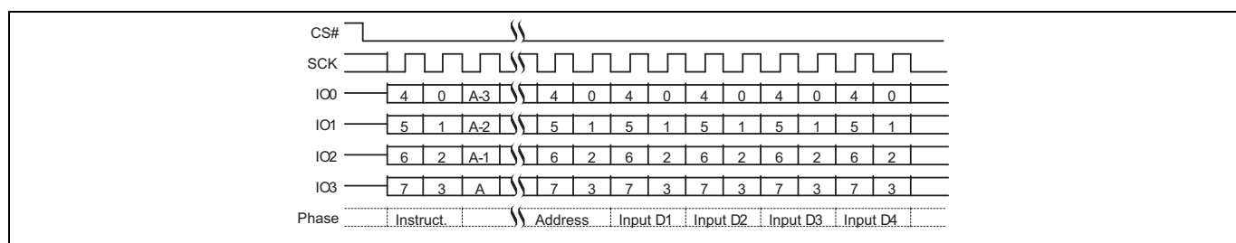
Figure 79 Page Program (PP 02h or 4PP 12h) QPI mode command sequence [64]
