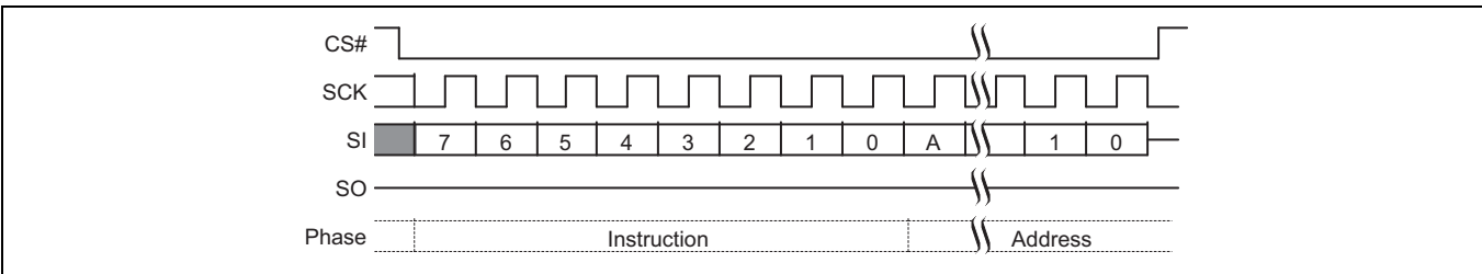
Figure 86 EES command sequence [66]
