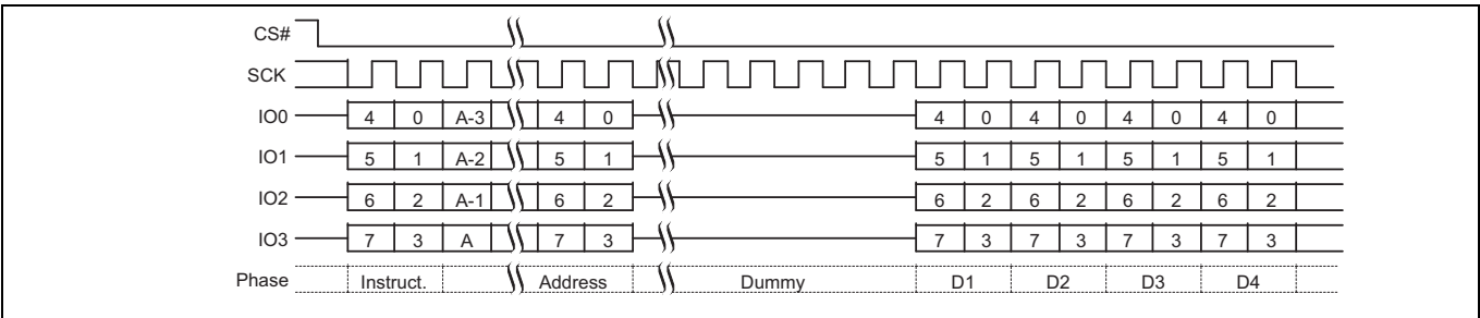
Figure 66 Read Any Register, QPI Mode, command sequence [50]
