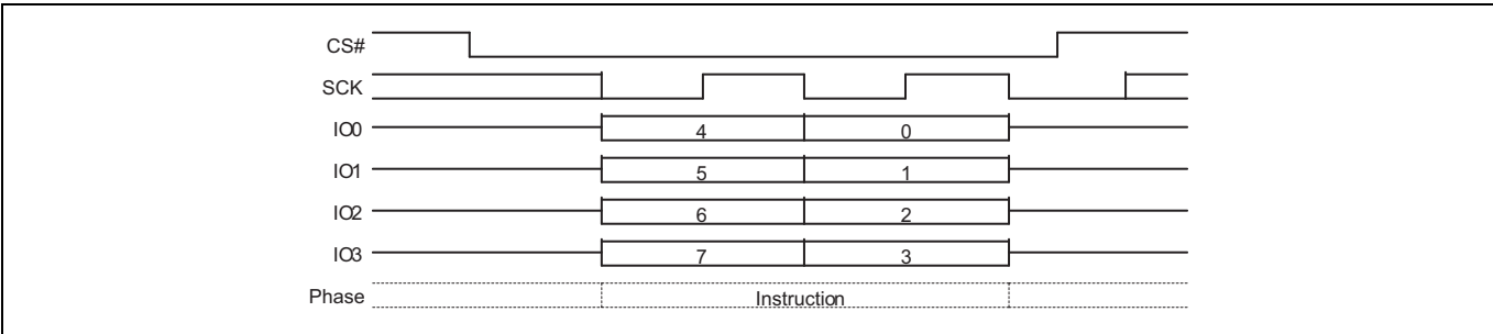
Figure 114 RES command sequence QPI mode
