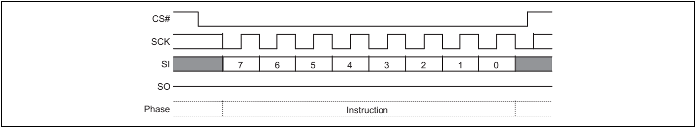
Figure 56 Clear Status Register (CLSR) command sequence
