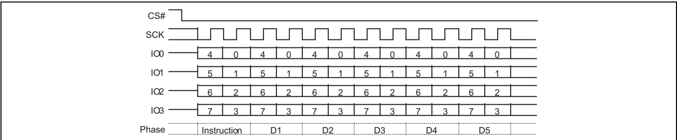
Figure 41 Read Identification (RDID) QPI mode command
