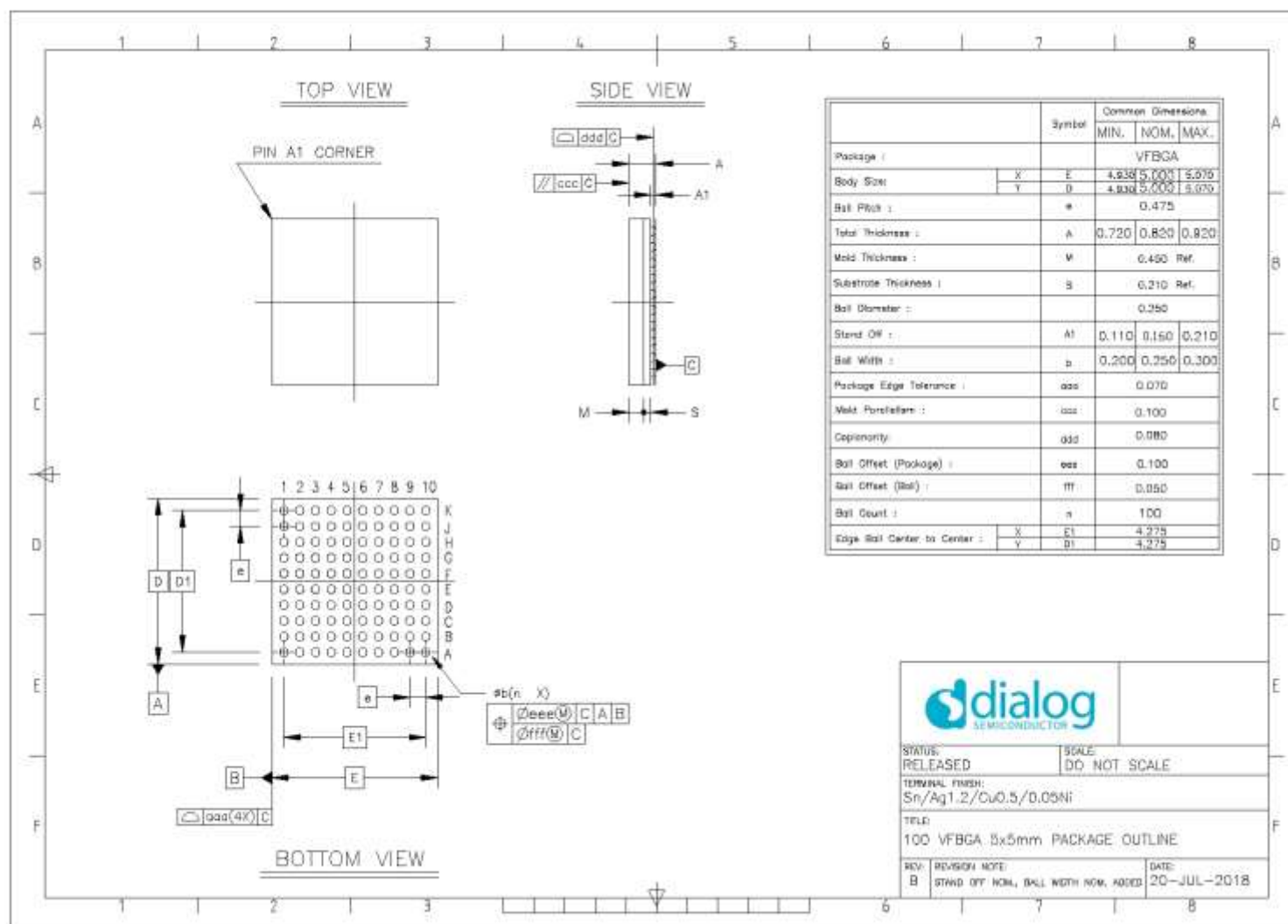
Figure 112: VFBGA100 Package Outline Drawing
