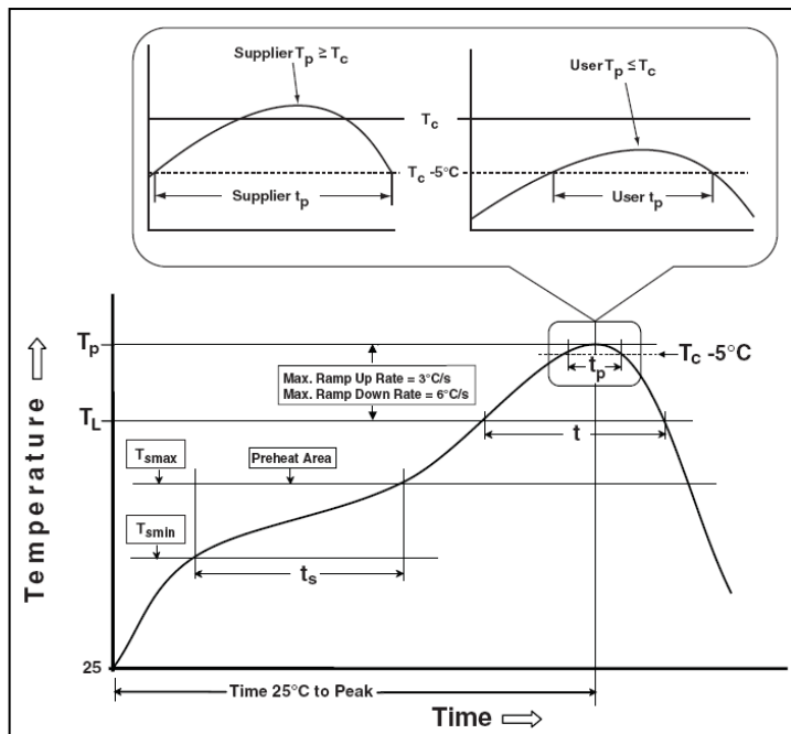
Figure 14 Classification Profile
