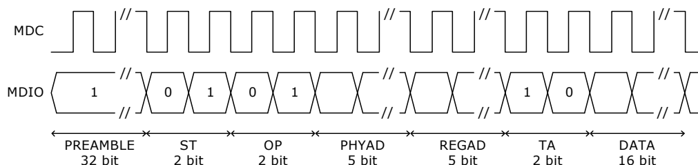
Figure 136 • MIIM Slave Write Sequence
