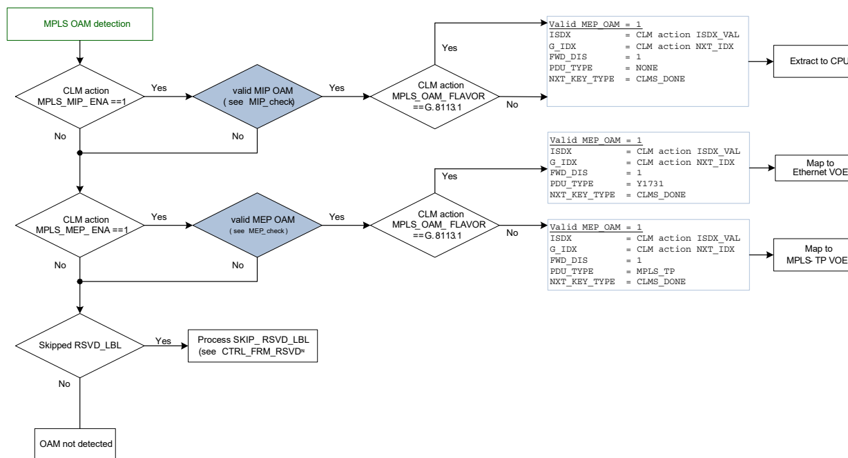
Figure 27 • MPLS OAM Detection
