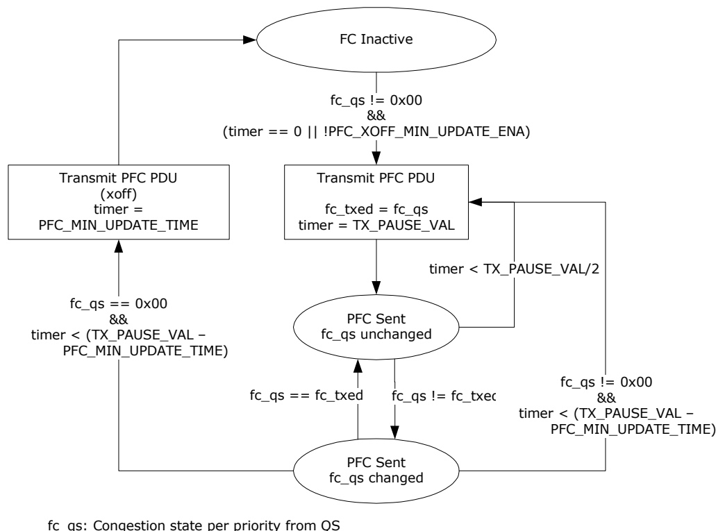
Figure 126 • PFC Generation per Port
