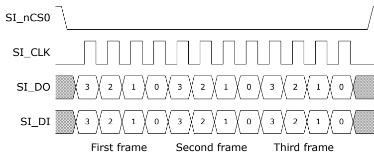
Figure 148 • SIMC SPI 3x Transfers
