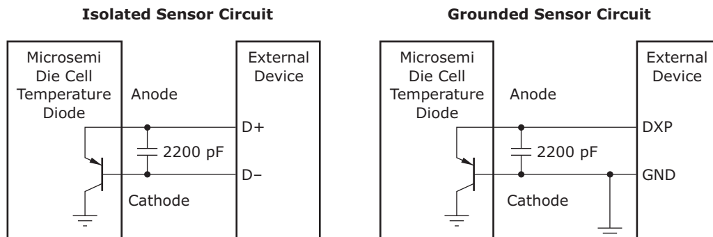
Figure 162 • Thermal Diode
