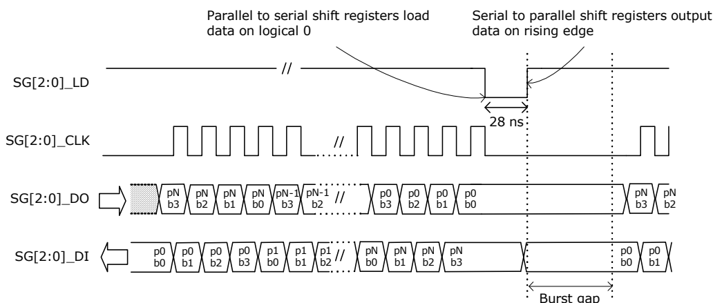
Figure 153 • SIO Timing
