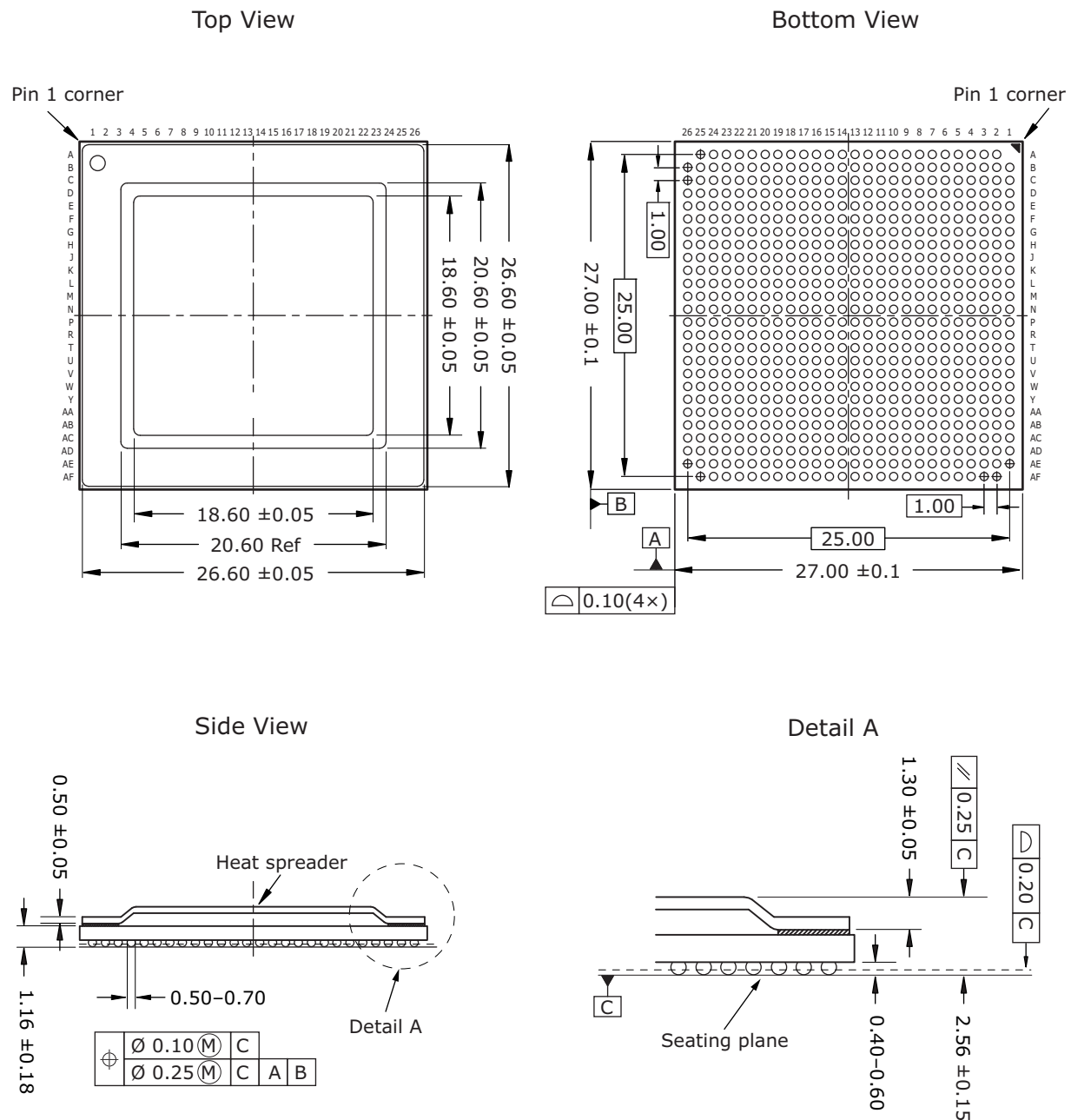
Figure 186 • Package Drawing
