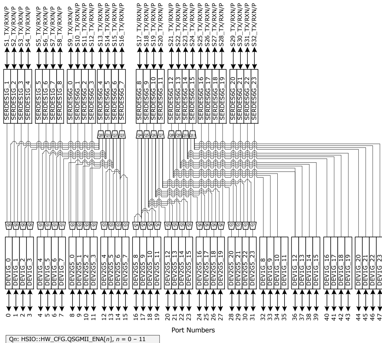
Figure 16 • QSGMII Muxing
