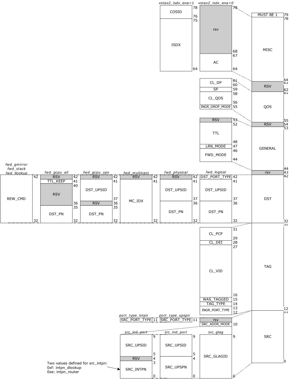
Figure 15 • VStaX Header Layout
