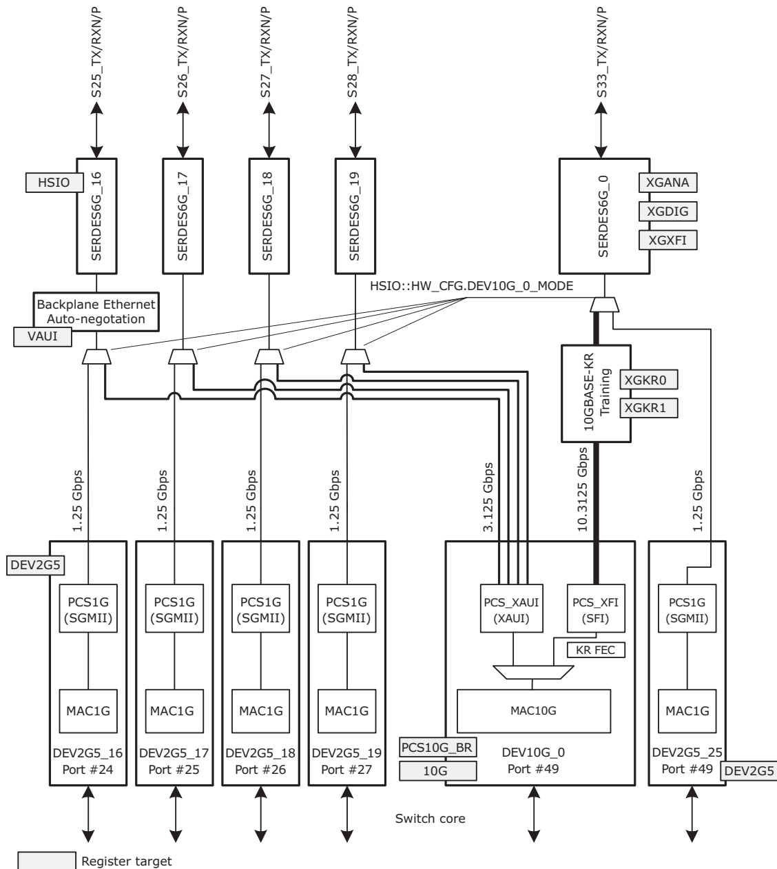
Figure 17 • 10G Muxing
