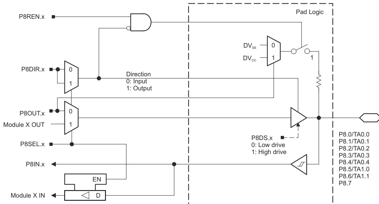
Figure 9-15. Port P8 (P8.0 to P8.7) Diagram
