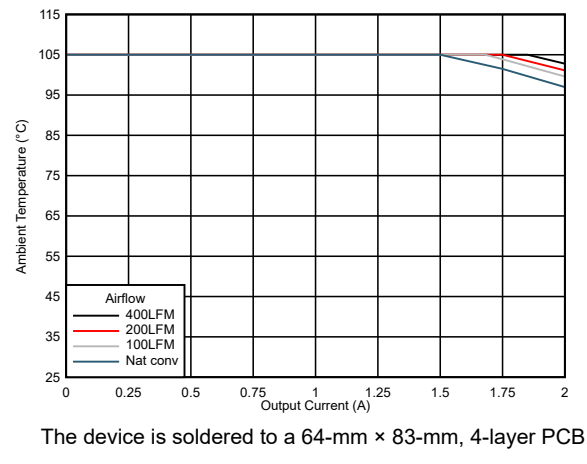
Figure 7-20. Safe Operating Area ( V_{OUT} = 3.3\text{ V} )
