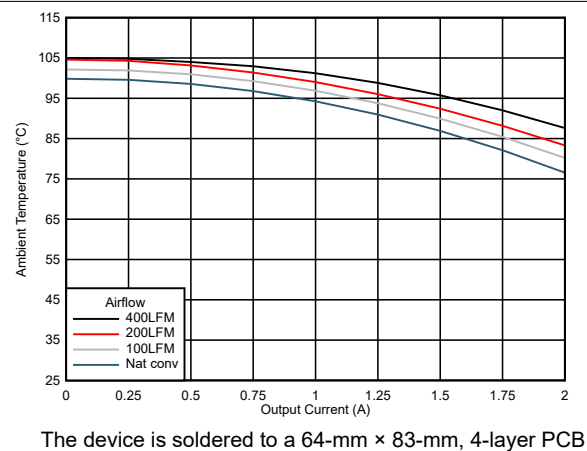
Figure 7-22. Safe Operating Area ( V_{OUT} = 12\text{ V} )
