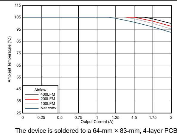
Figure 7-21. Safe Operating Area ( V_{OUT} = 5.0\text{ V} )
