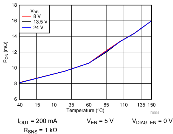
Figure 7-5. On Resistance ( R_{ON} ) vs Temperature
