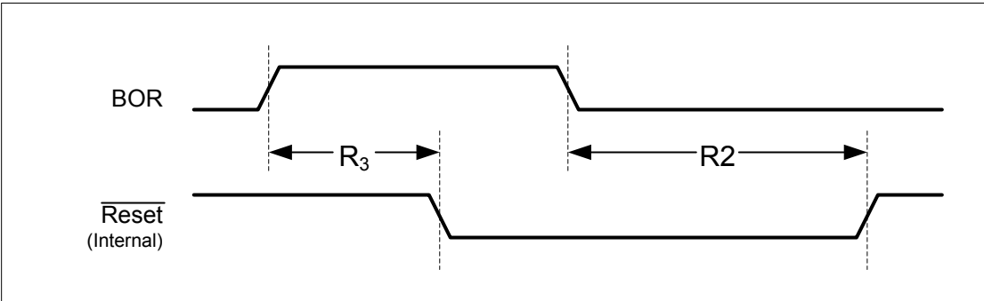
Figure 30-11. External Reset Timing ( \overline{\text{RST}} )
