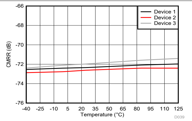
Figure 6-30. Common-Mode Rejection Ratio vs Temperature f_{IN} = 10 kHz
