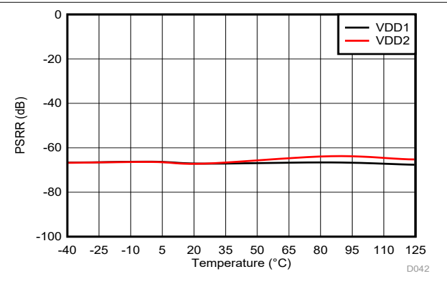
Figure 6-32. Power-Supply Rejection Ratio vs Temperature f_{Ripple} = 10 kHz
