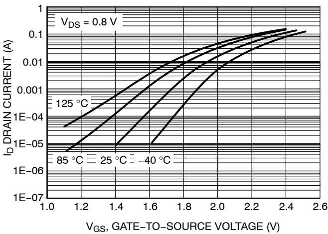
Figure 8. Transfer Function
