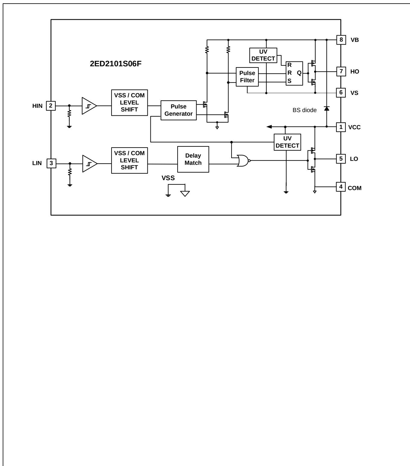
Figure 2 Block diagrams
