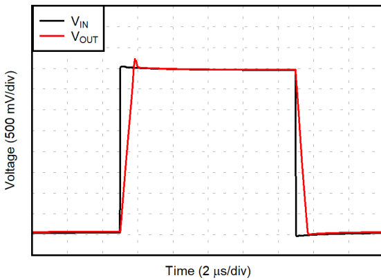
Figure 6-31. Large-Signal Step Response (4-V Step)
