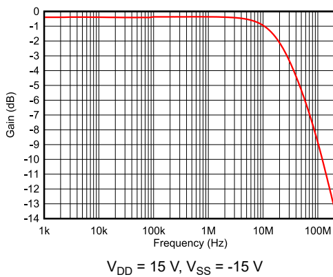
Figure 7-27. On Response vs Frequency
