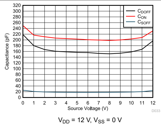
Figure 7-30. Capacitance vs Source Voltage or Drain Voltage
