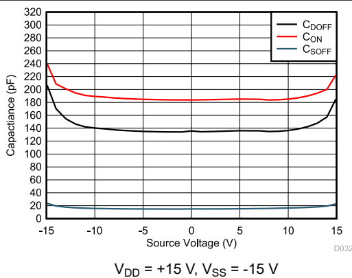
Figure 7-29. Capacitance vs Source Voltage or Drain Voltage
