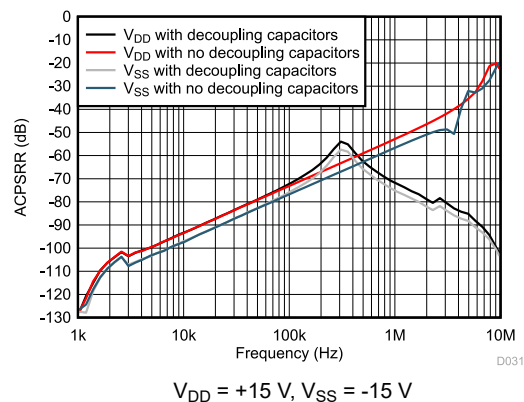
Figure 7-28. ACPSRR vs Frequency
